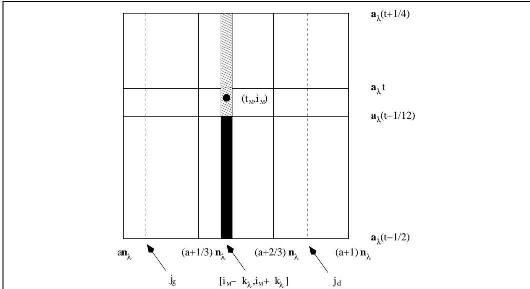
FIGURE 7. The event \Omega_{a,t}^\lambda .
