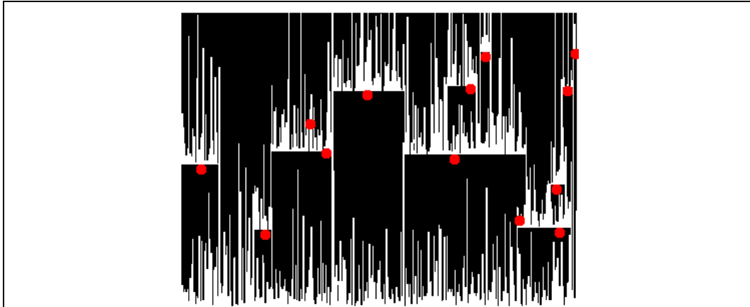
FIGURE 12. Simulation with \beta = 5 .
