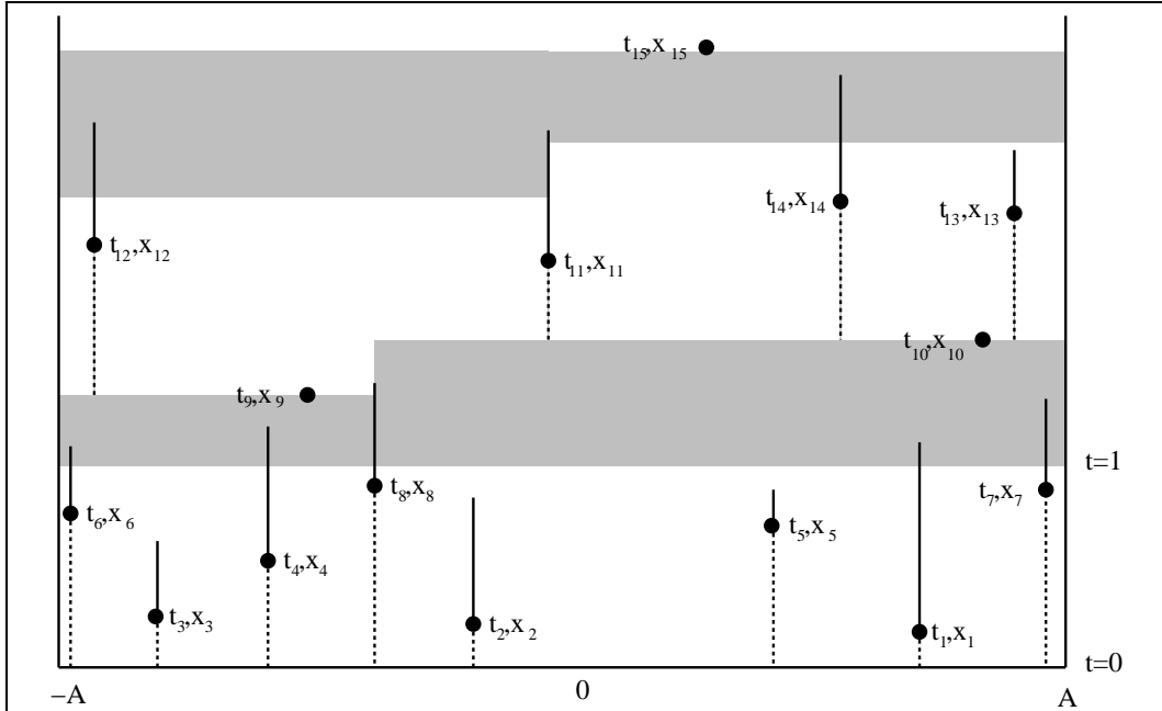
FIGURE 3. LFF(BS) -process in a finite box.
