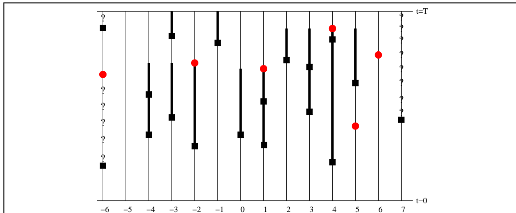
FIGURE 1. Graphical construction of the FF(\mu_S, \mu_M) -process.
