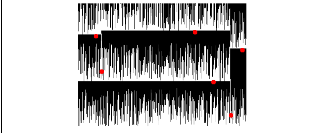
FIGURE 10. Simulation with \beta = BS .
