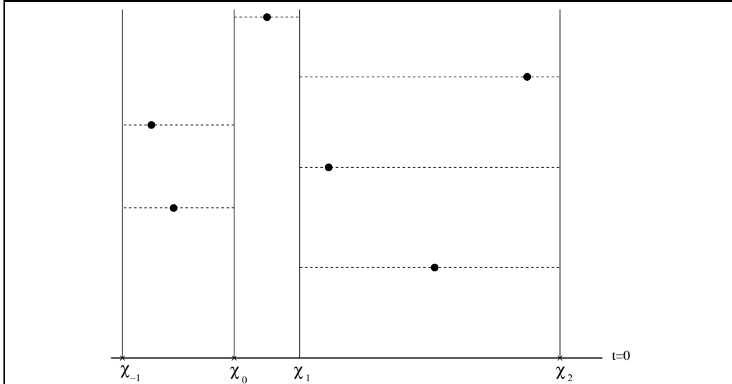
FIGURE 5. LFF(0) -process.
