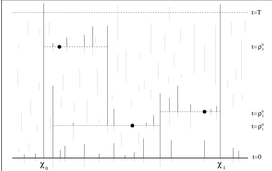
FIGURE 4. LF\!F(\beta) -process with \beta \in (0, \infty) .
