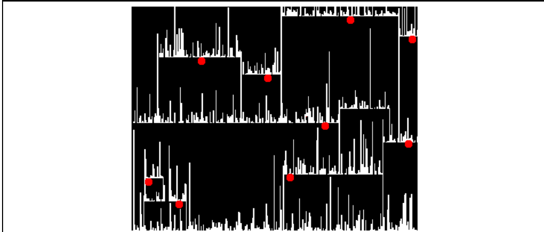
FIGURE 13. Simulation with \beta = 2 .
