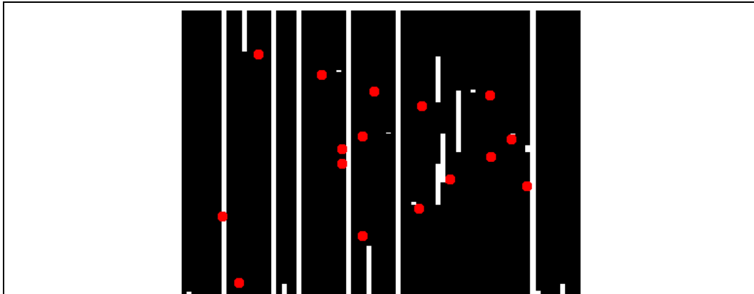
FIGURE 14. Simulation with \beta = 0 .
