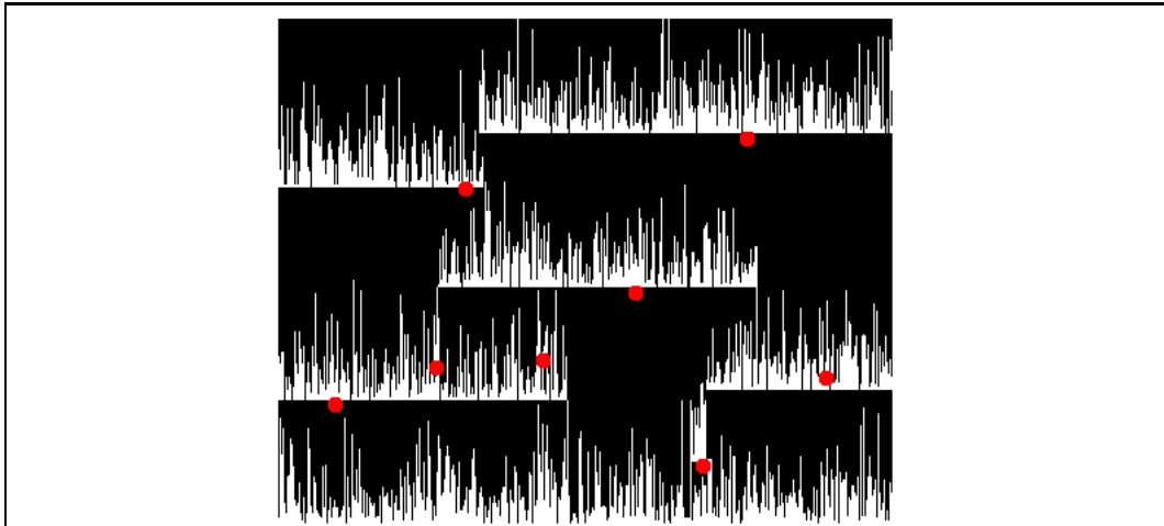
FIGURE 11. Simulation with \beta = \infty .
